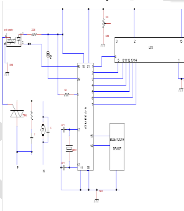
Figure 4: Basic circuit diagram
