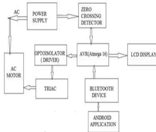
Figure 2: Block Diagram
