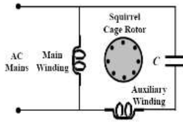
Figure1: Capacitor run single phase induction motor
