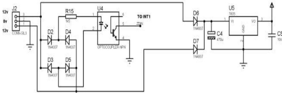
Figure 3: zero crossing detector
