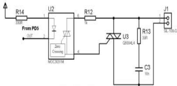
Figure 5: firing angle circuit
