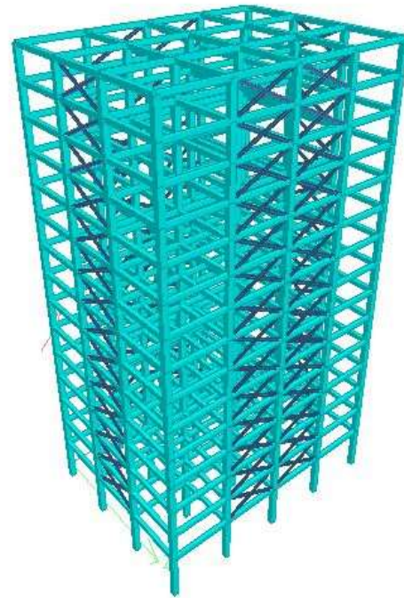
FIG.-5 CROSS BRACING AT MID BAY
