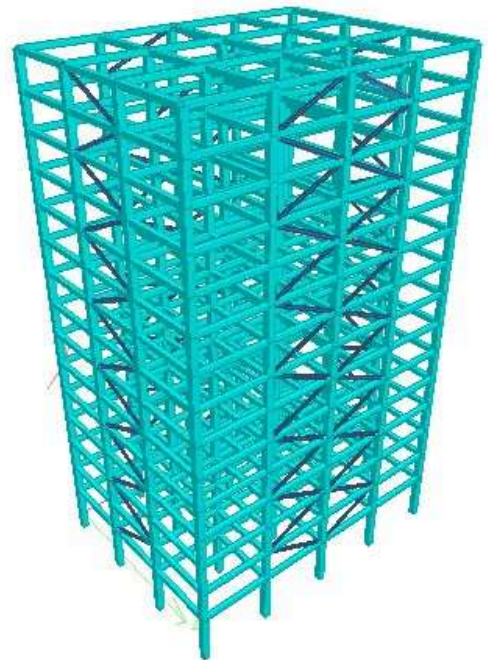
FIG.-7 DIAGONAL BRACING AT MID BAY
