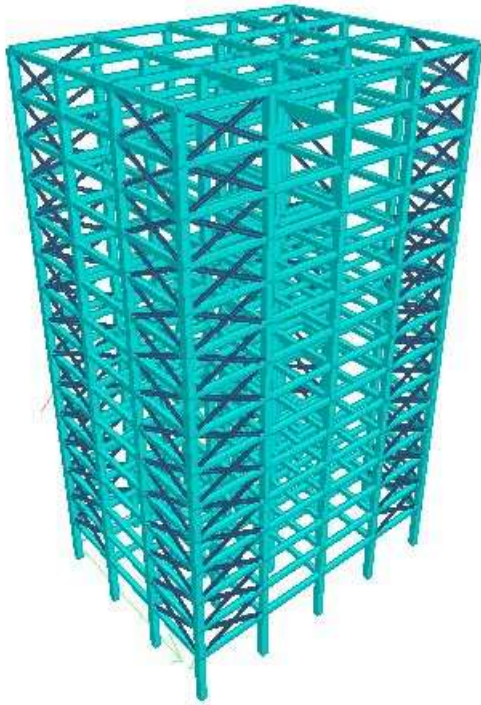
FIG.-4 CROSS BRACING AT CORNER
