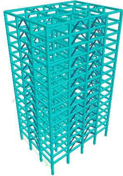
FIG.-9 INVERTED V BRACING AT MID BAY
