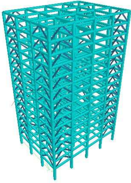
FIG.-8 INVERTED V BRACING AT CORNER
