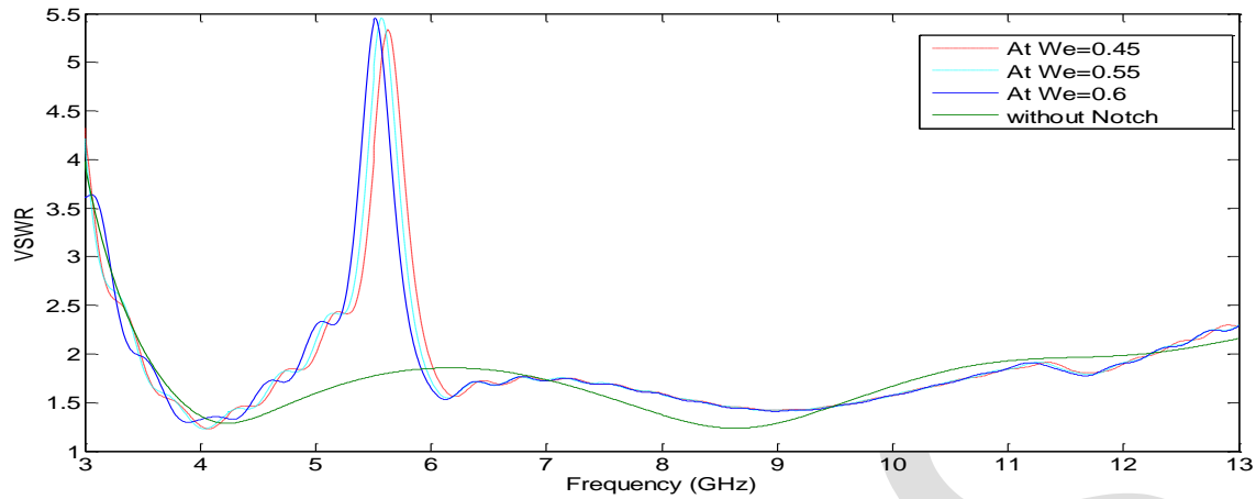
Fig 4 VSWR vs. Frequency plots with and without Notch
