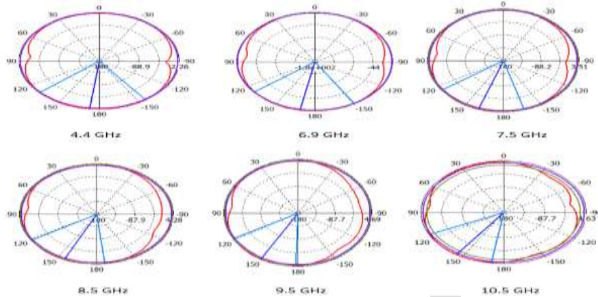
Fig 6 Radiation patterns for antenna with notches
